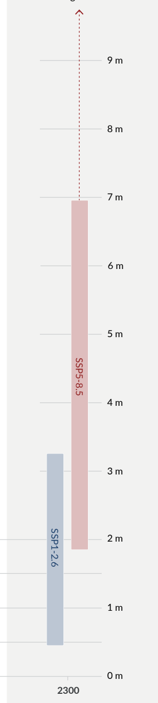
Figure SPM.8 | Selected indicators of global climate change under the five illustrative scenarios used in this Report
